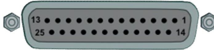
View of Socket on VBOX III
